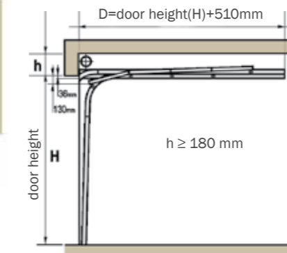
LHR FM low headroom lift double tracks, front mounted springs
