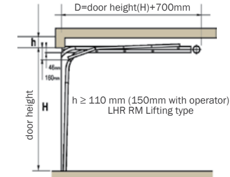
LHR RM low headroom lift double tracks, rear mounted springs
