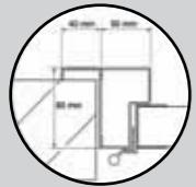
Frame domentions
